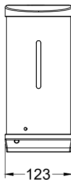
Front view
